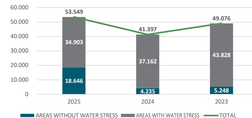
Water withdrawals by exposure to water stress (m 3 )
