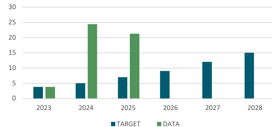
Renewable energy consumption (%)
