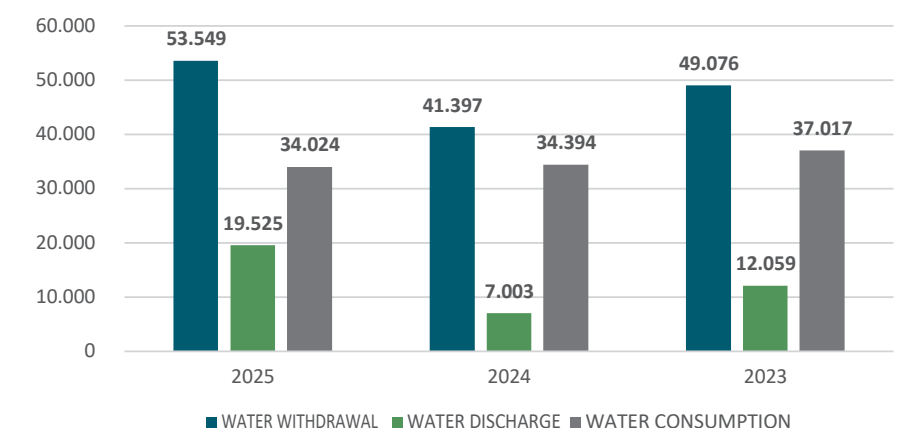
Water withdrawals, discharges and consumption (m 3 )
