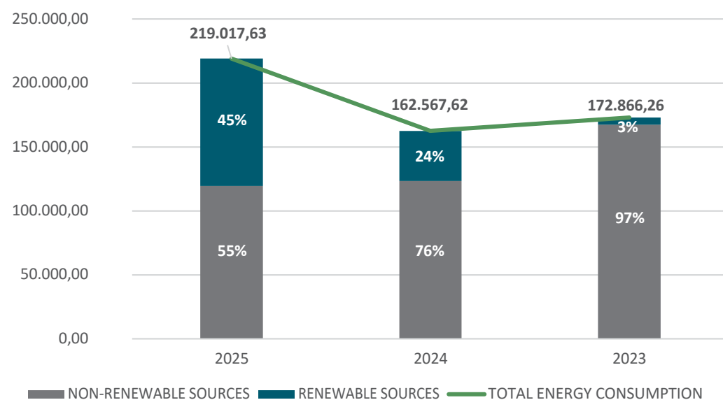
Total energy consumption (GJ)
